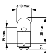
R5W (BA15d)
