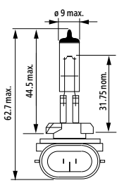
H27W/2 (881)
