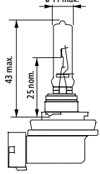
H27W/2 (881)
