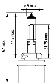
H27W/1 (880)
