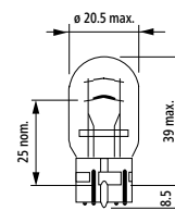
W21/5W
