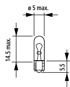
W1,2W, W2,3W
