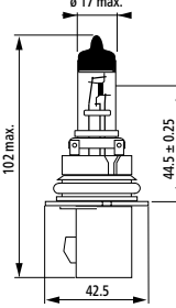
HB5 (9007)
