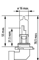
HB3 (9005)
